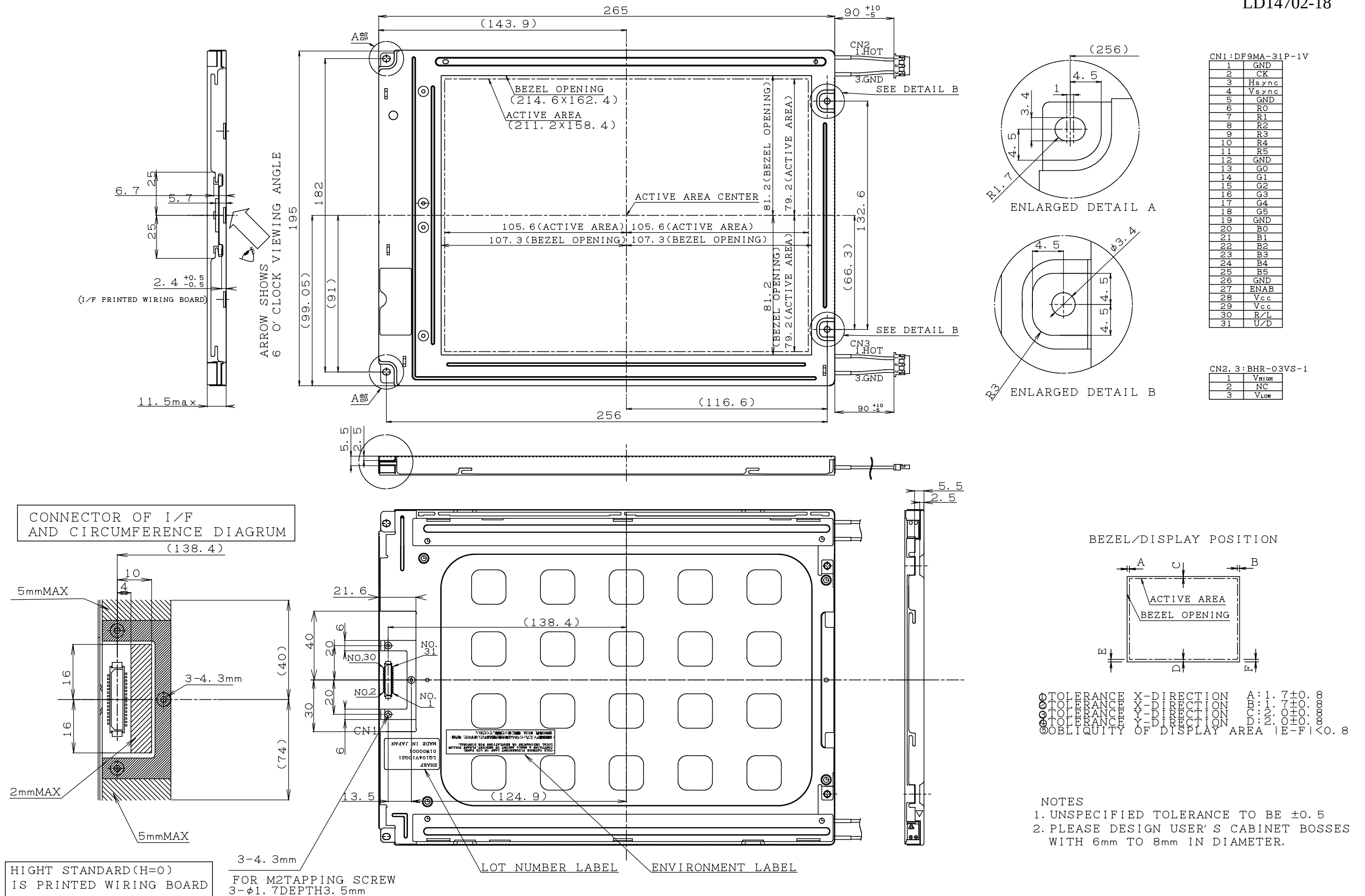
Fig.1 Outline Dimensions
